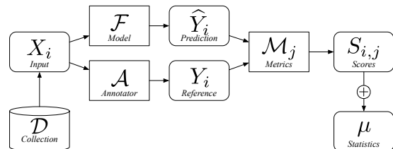
Figure 2. Diagram of the standard approach to the benchmarking of MIR systems.
